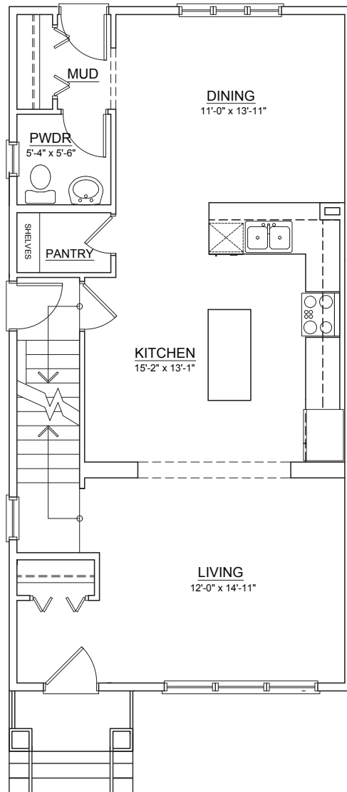
MAIN FLOOR ±830 SQ. FT.
